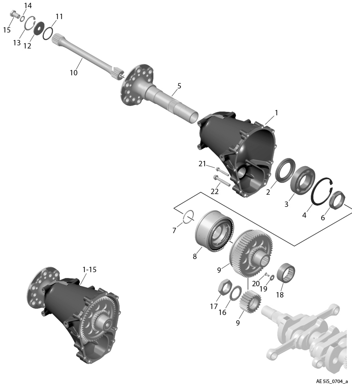
Figure 5.1: Propeller gear assy.
