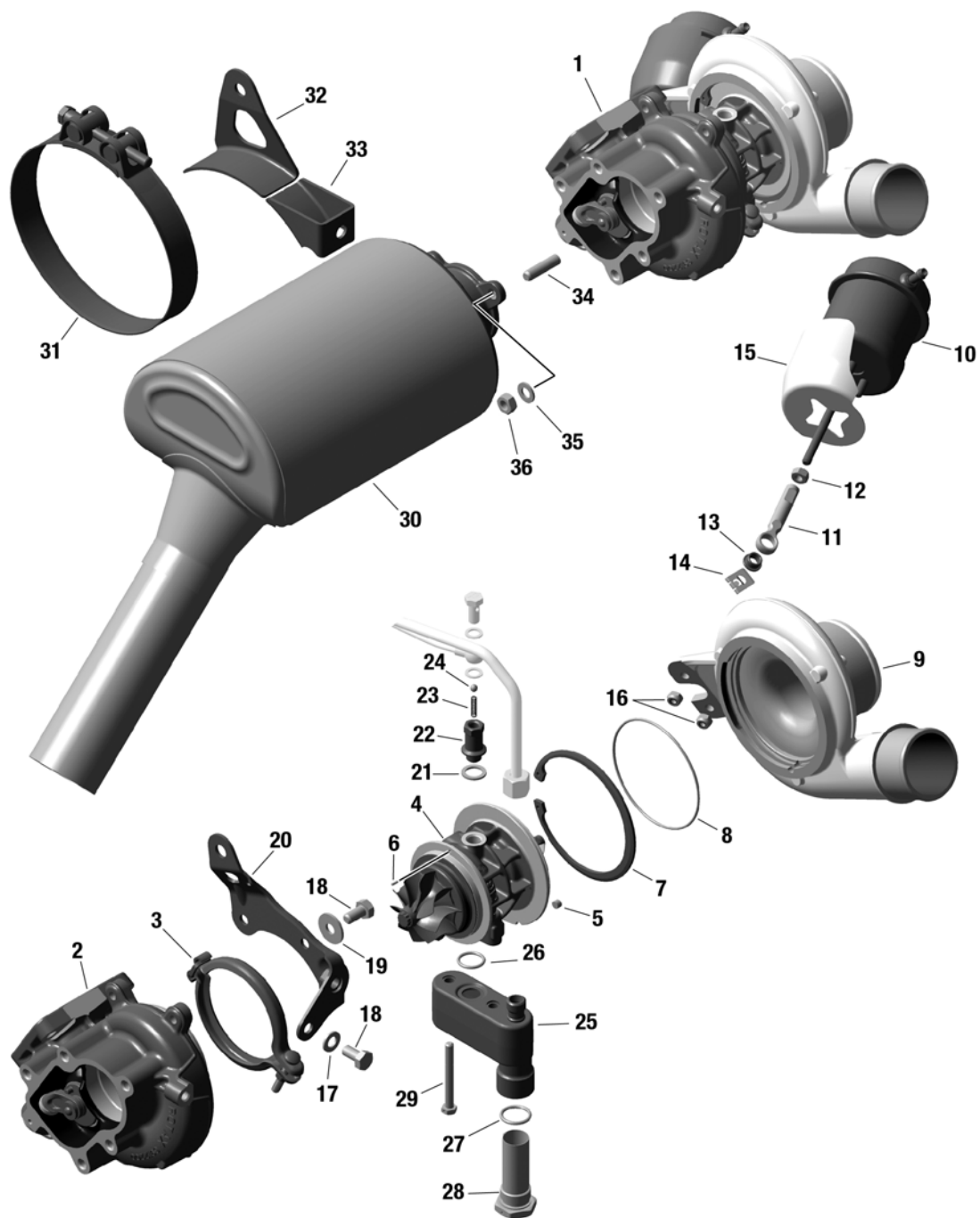
Figure 12.2: 78-10-00, TURBOCHARGER MY20
