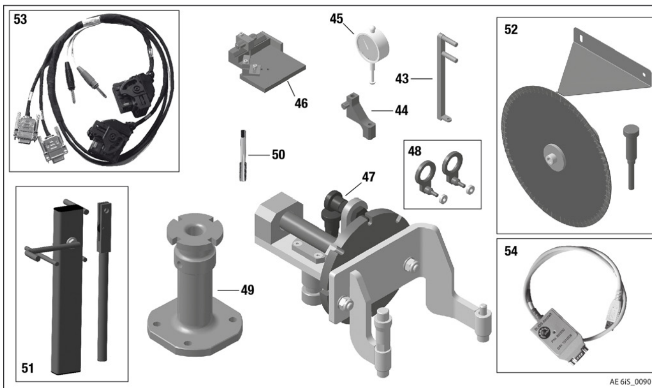
Figure 1.6: Repair tools
