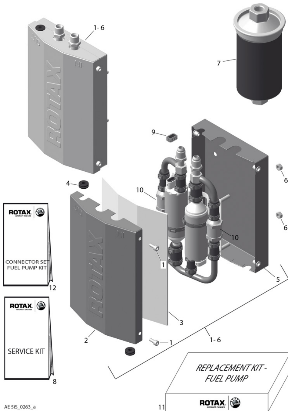
Figure 7.4: 73-10-00
