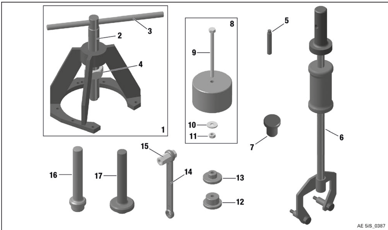
Figure 1.3: Repair tools
