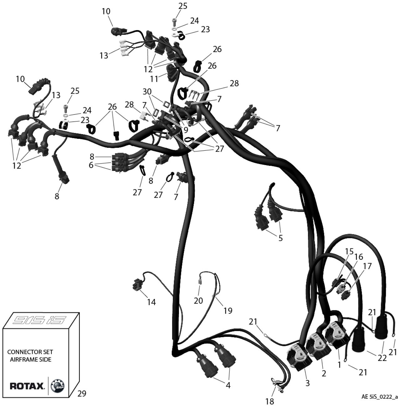
Figure 11.1: 76-50-00
