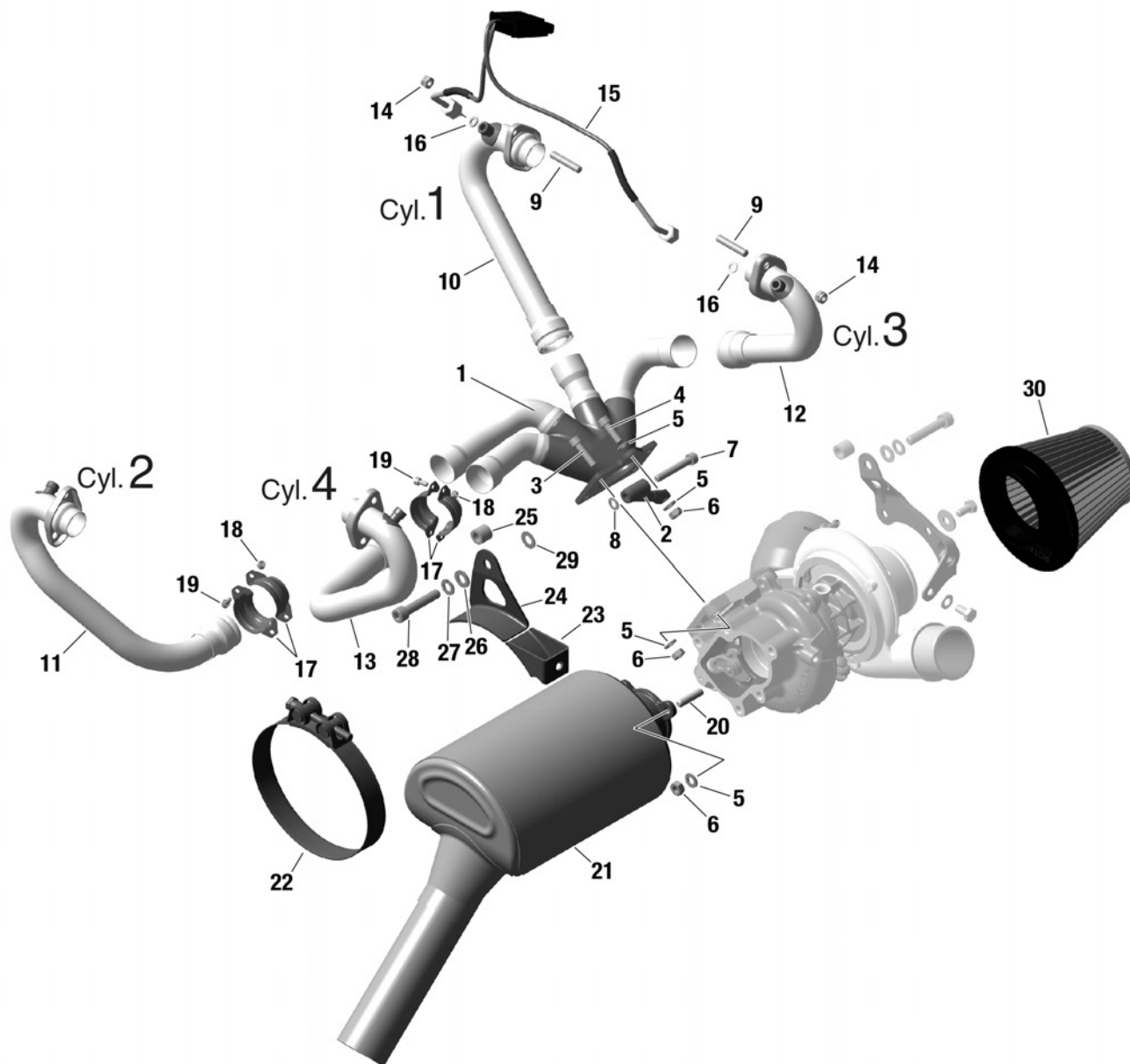
Figure 12.1: 78-10-00
