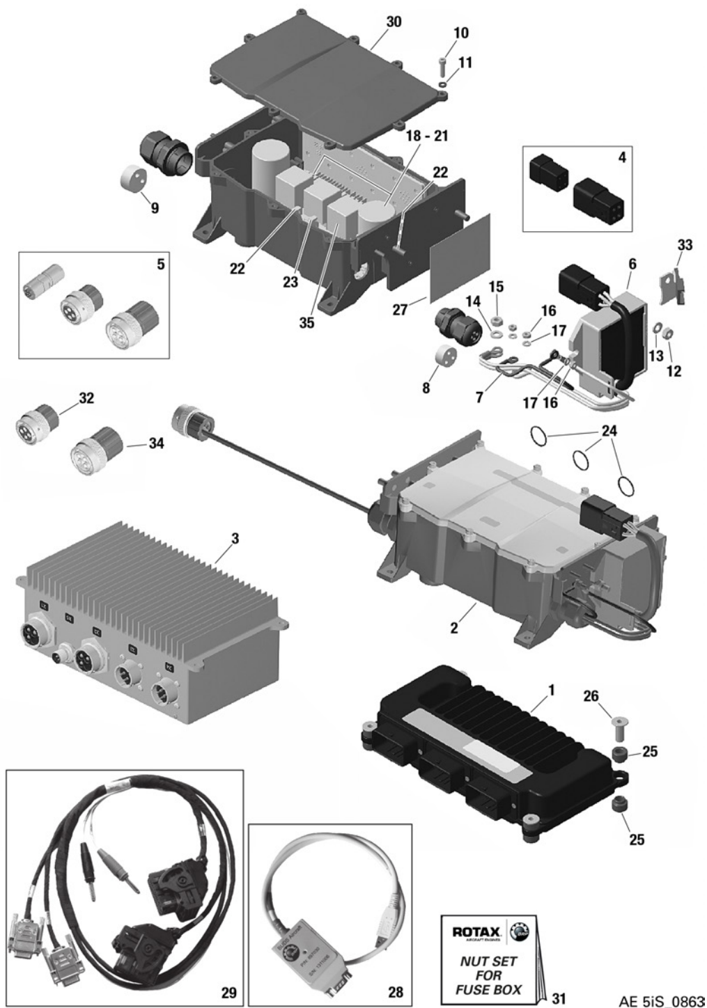
Figure 10.1: 76-10-00
