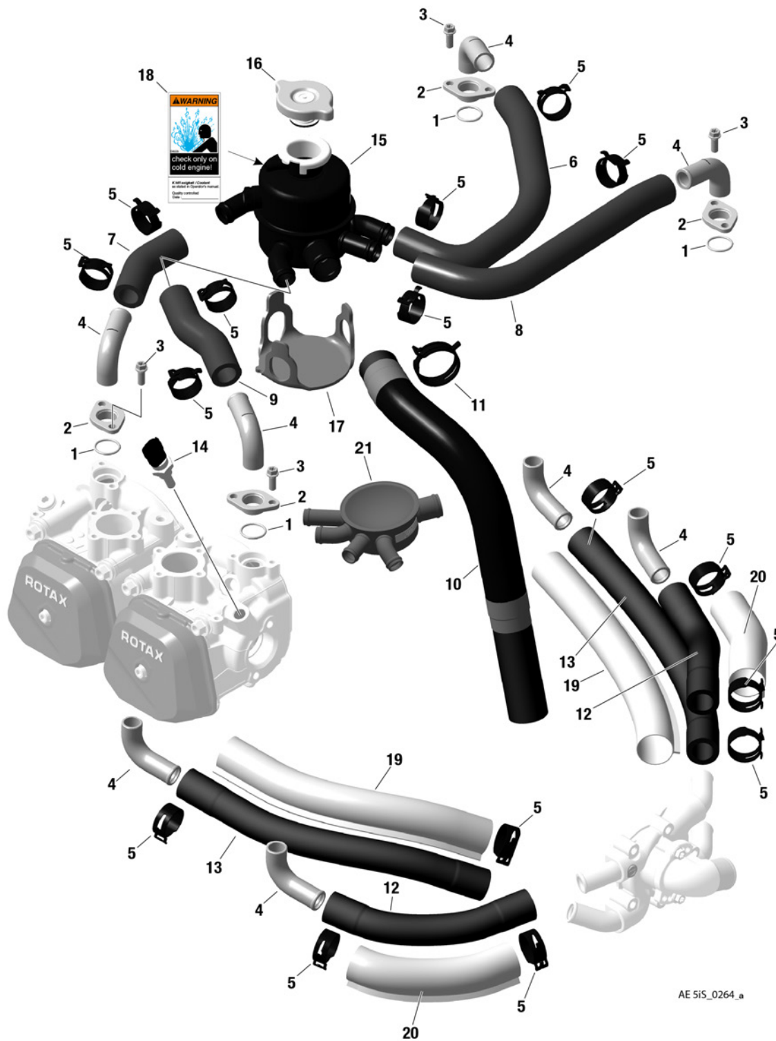
Figure 9.2: 75-20-00
