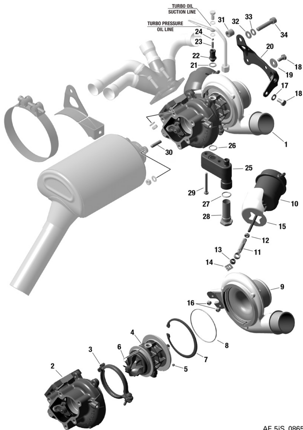
Figure 12.2: 78-10-00, TURBOCHARGER MY20
