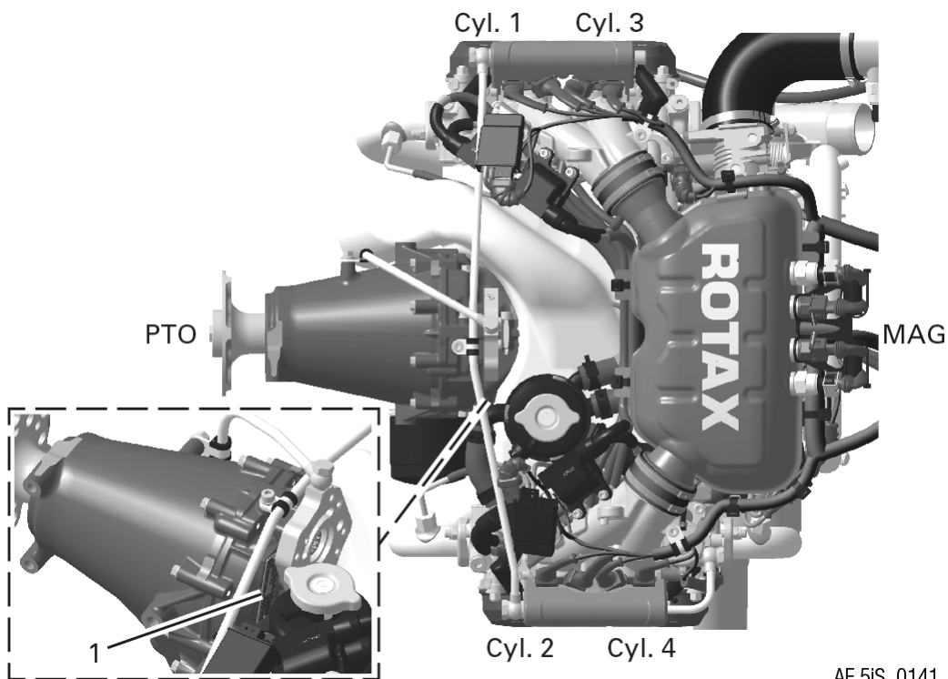
Figure 1.1: Engine view, TYPICAL
