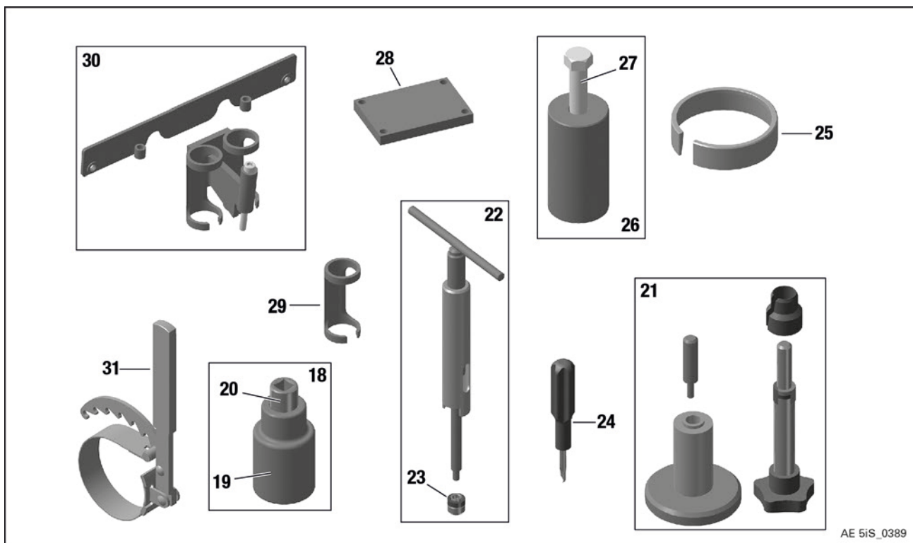
Figure 1.4: Repair tools
