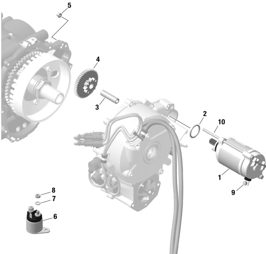
Figure 14.1: 80-10-00
