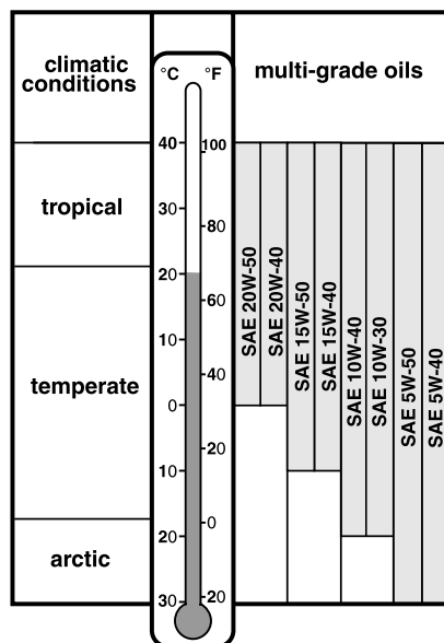
Figure 1: Temperature range
