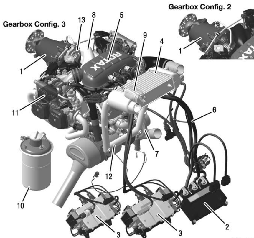
Figure 1: Engine components
