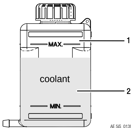
Figure 2: Overflow bottle
