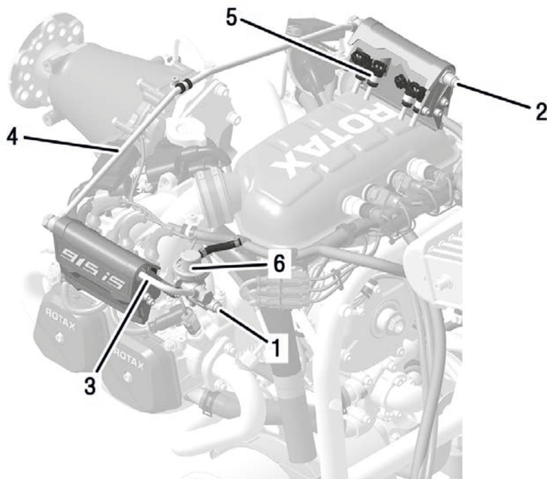
Figure 5: Fuel system
