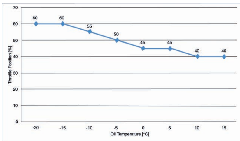
Figure 3: Throttle position
