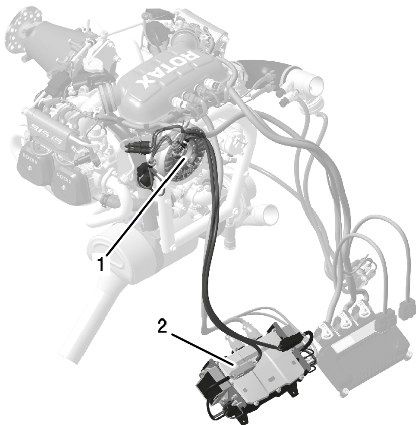
Figure 8: Internal power supply
