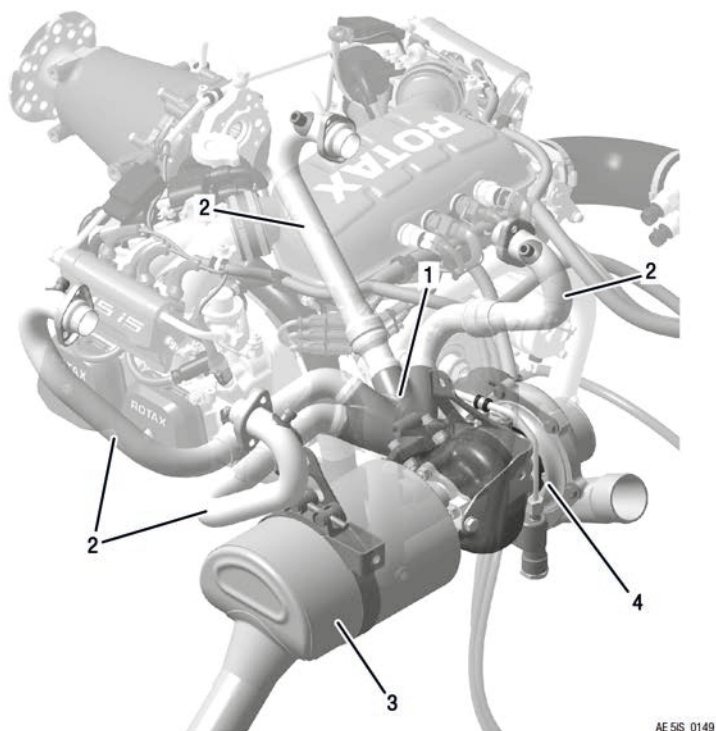
Figure 12: Turbocharger/Exhaust system
