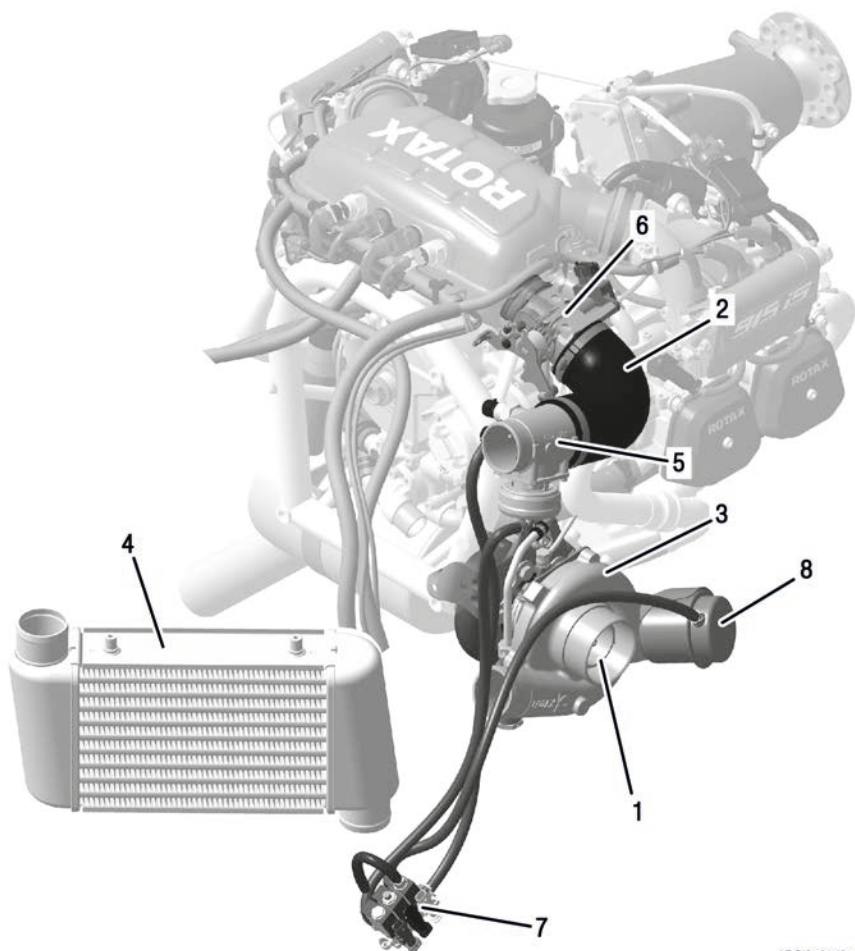
Figure 10: Air intake system
