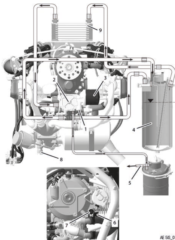
Figure 7: Lubrication system
