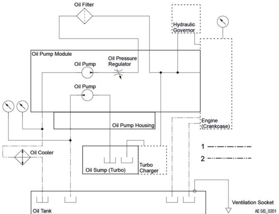
Figure 6: Lubrication system (symbolic)
