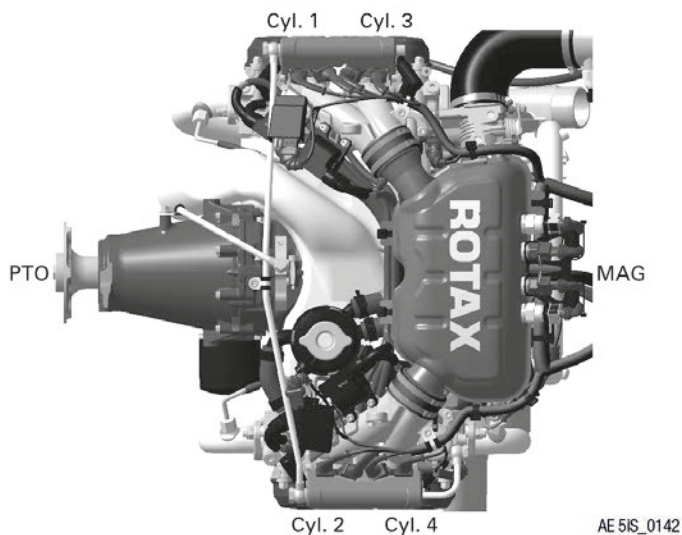
Figure 2: Cylinder arrangement
