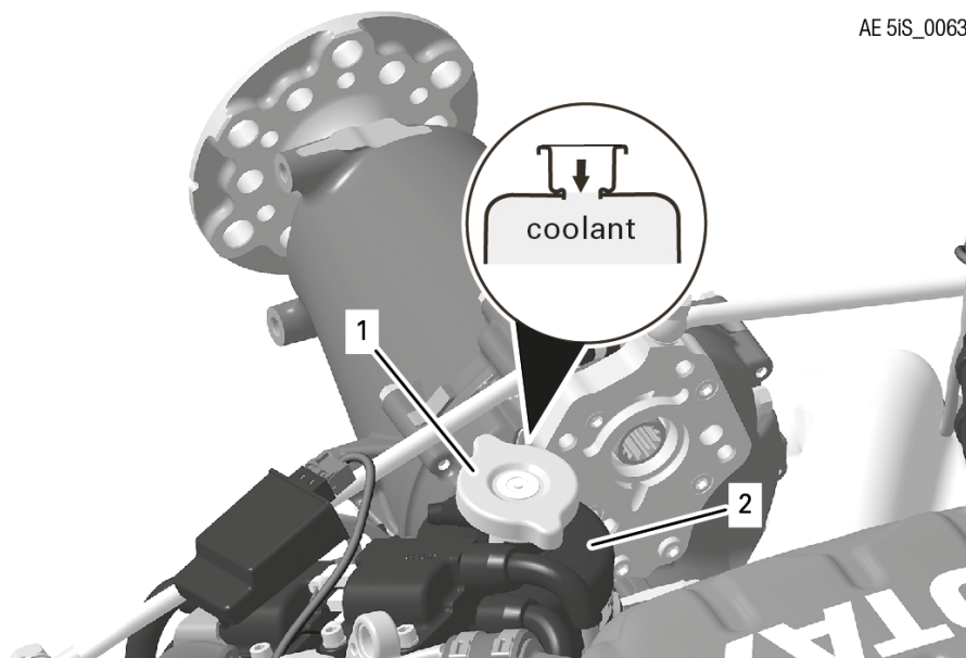
Figure 1: Expansion tank
