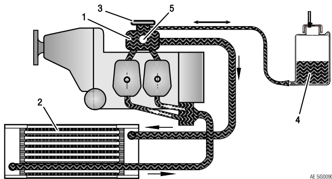
Figure 4: Cooling system (symbolic)
