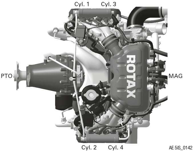
Figure 3: Cylinder arrangement
