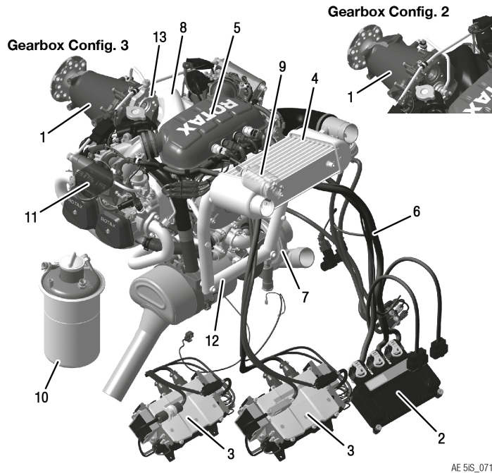
Figure 1: Engine components
