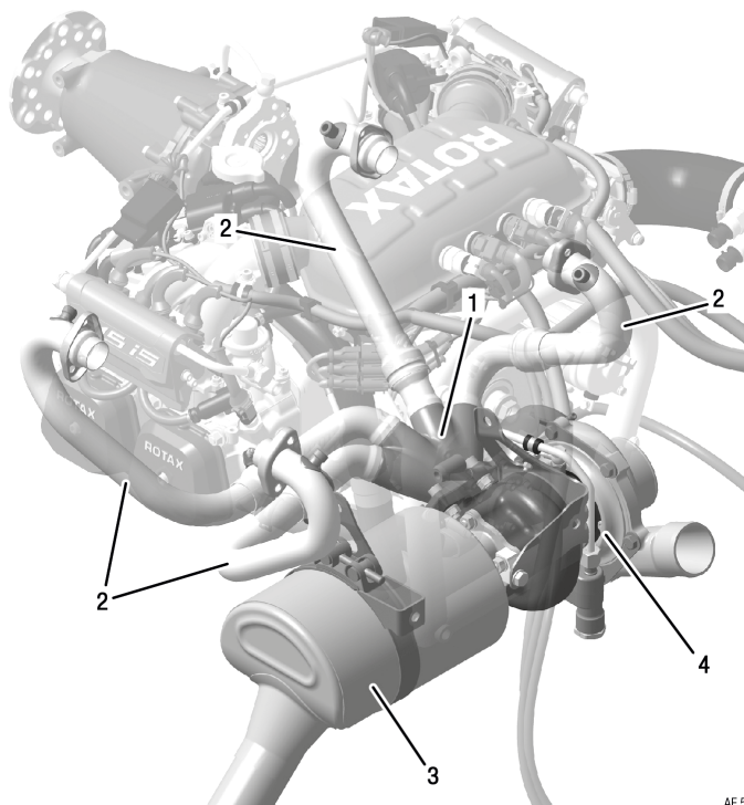
Figure 15: Turbocharger/Exhaust system
