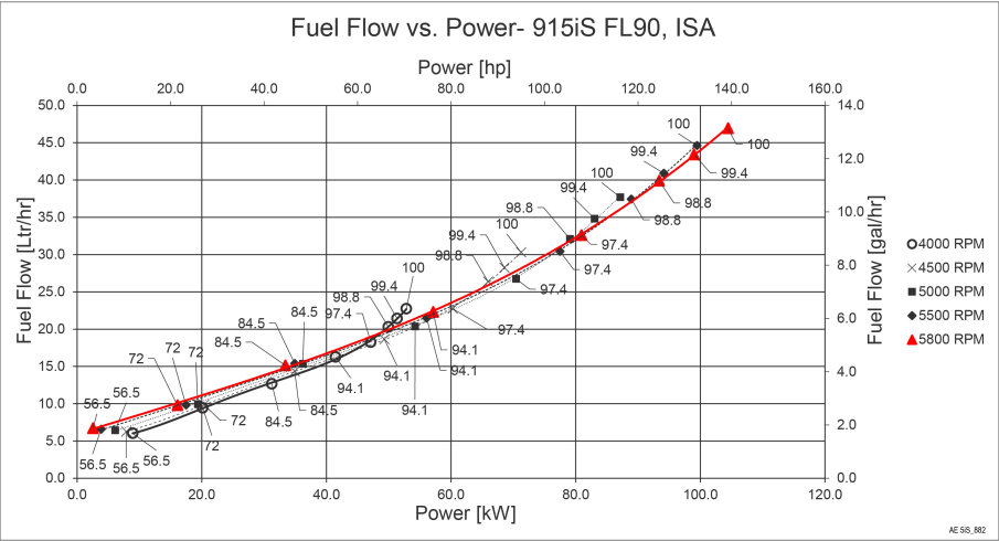
Figure 6: Fuel flow
