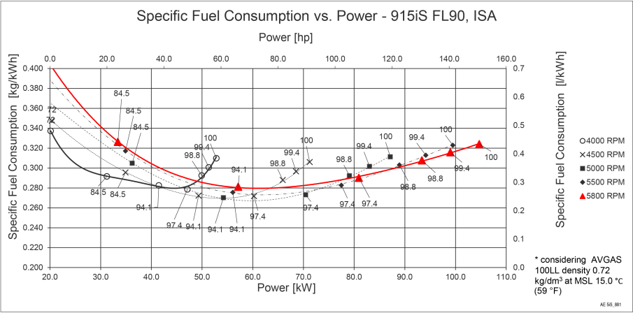
Figure 5: Specific Fuel Consumption
