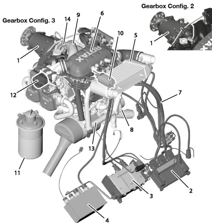
Figure 2: Engine components
