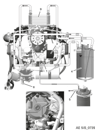
Figure 8: Lubrication system
